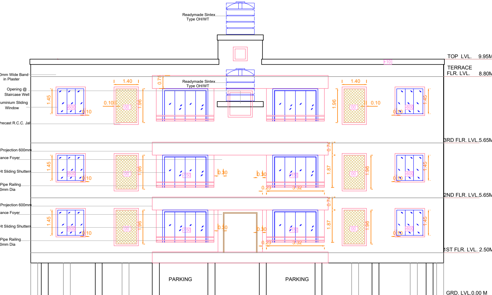
TYPICAL FRONT ELEVATION SOUTH FACE
