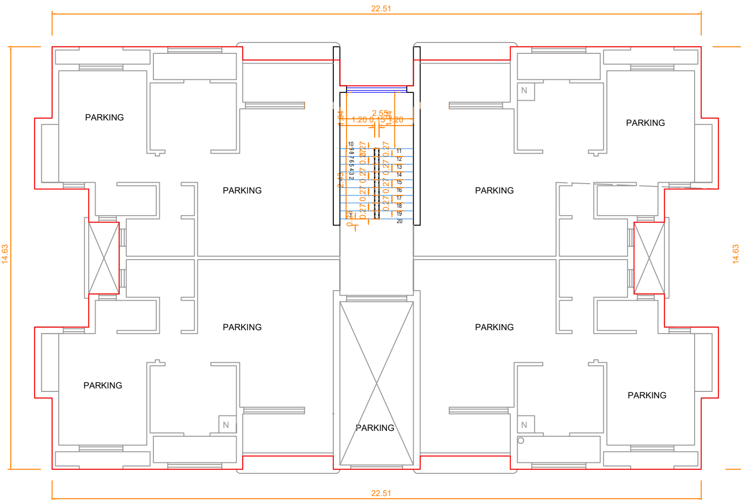
PROPOSED STILT / PARKING FLOOR PLAN
