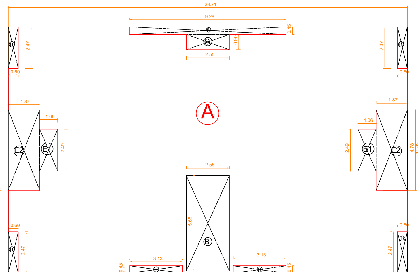
BLOCK PLAN TYPICAL G+2
