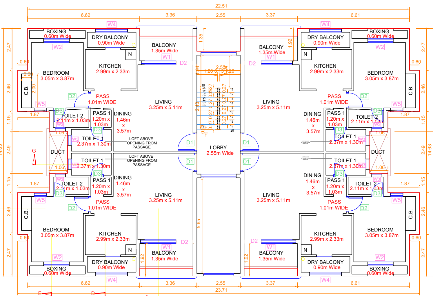
PROPOSED 2ND FLOOR PLAN
